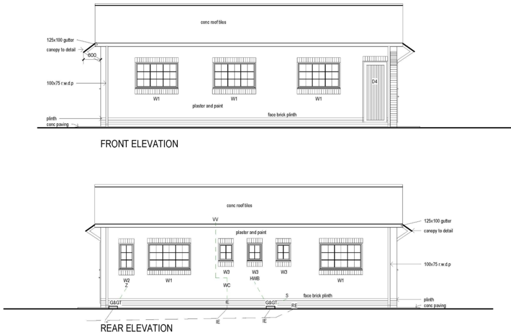
Figure 1: Elevation drawings of the planned house for 3 teachers.
